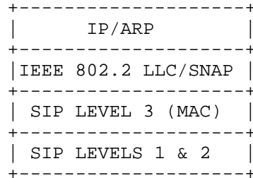
Figure 1. Protocol stack for IP over SMDS Service
