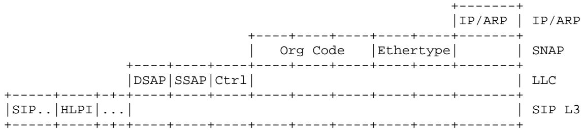
Figure 2. Data Link Encapsulation
